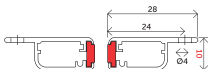
Profilo meccanico / Mechanical profile
